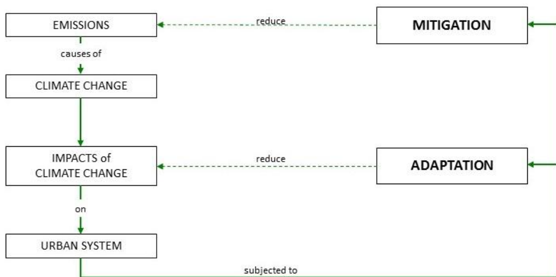
Fig. 1 - Relations between urban system, climate changes, mitigation and adaptation (elaborated by Fussler et al., 2006).
